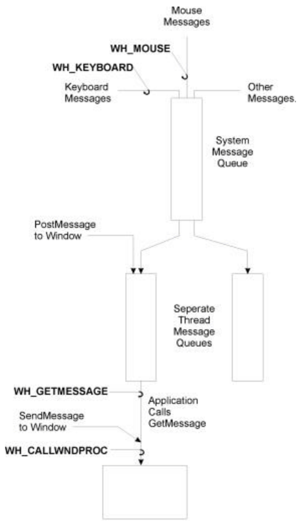
Figure 4 Message Flow and Hooks
